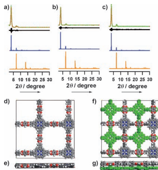
Figure 3. XRD patterns of H 2 P-COF (a), ZnP-COF (b), and CuP-COF (c). The experimentally observed: green; the Pawley refinement: red; their difference: black; the simulation of achiral AA stacking model: blue; the simulation of AB stacking model: orange. Views of the unit cell derived from achiral AA stacking model along the z (d) and y (e) axes of ZnP-COF. Views of the unit cell derived from AB stacking model along the z (f) and y (g) axes of ZnP-COF.
